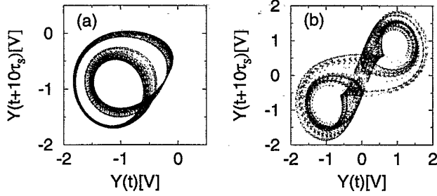
FIG. 2. The projections of attractors CA_X (a) and CA_Y (b) reconstructed by time delay embedding with time delay 10\tau_S . The sampling time \tau_S = 20 \mu\text{sec} .
