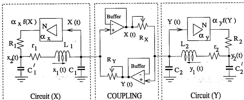
FIG. 1. Diagram of asymmetrically coupled chaotic circuits. N , nonlinear converter.
