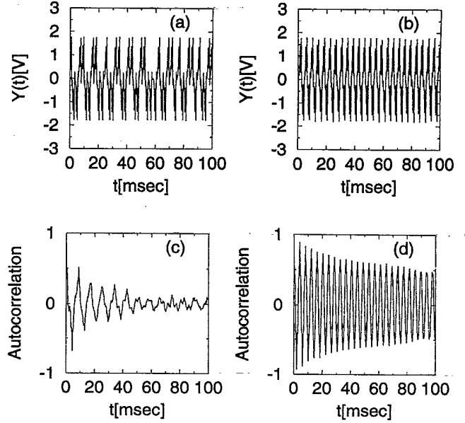
FIG. 4. The time series of Y(t) for (a) R_X = 77 \Omega and (b) R_X = 106 \Omega . (c) and (d) are the corresponding autocorrelation functions.
