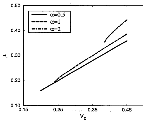
FIG. 4. Control amplitude versus v_0 for different values of the form-factor width \alpha . Control fails to the left of the graphs.
