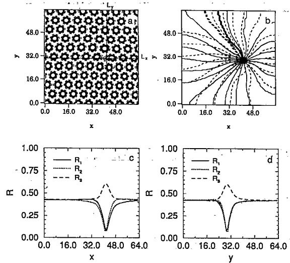
FIG. 4. “Penta-hepta” pair formed by merging of two dislocations: (a) isolines of the “temperature” field T = \sum_{i=1}^3 A_i \exp(ix_i) ; (b) equiphasic lines of \phi_1 (solid) and \phi_2 (dashed); (c) cross sections of the magnitudes R_i along the line L_x in (a); (d) the same as in (c) along the line L_y in (a).
