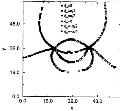
FIG. 3. Trajectories of the cores of dislocations in the hexagonal pattern for several different phase shifts between roll systems \phi_0 .
