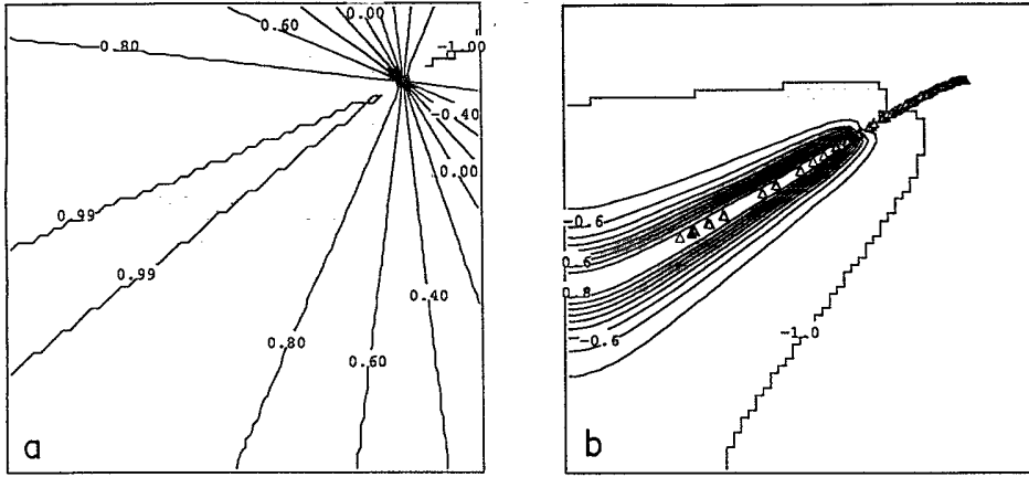
FIG. 1. (a) Profile of synchronization parameter F = -\cos\Phi for one dislocation in the hexagonal pattern at t=0 . (b) The same as in (a) for t=10 and the trajectory of the dislocation core (triangles, arrow shows the direction of defect motion).
