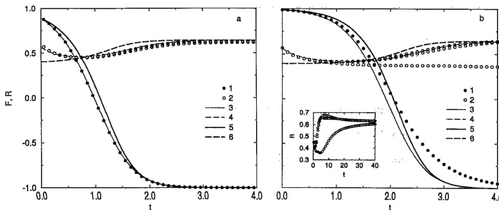
FIG. 5. Time dependence of amplitudes R_{1,2,3} and synchronization parameter F in two different space locations: (a) x=40, y=30 (outside the corridor), (b) x=40, y=20 (near the axis of the corridor). Symbols 1,2 show the results of numerical simulations of F (solid circles) and all three R_i (open circles) for the full set of amplitude equations (3) with \mu=1, \gamma=1.5 and initial condition (6) with R_{1,2,3}^0=0.65 , lines 3,4 show the corresponding solutions of the system (7),(11), and lines 5,6 show the results of the phase approximation (8),(12). The inset in (b) shows the long-term evolution of three amplitudes.
