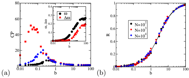
FIG. 2: Gillespie simulations of coupled stochastic oscillators: coherence parameter CP = \Delta\omega/\omega (a) and order parameter R (b) vs. b for N = 10^2, 10^3, 10^4 . Solid line in (b) is (8). Inset: frequency \omega and bandwidth \Delta\omega vs. b .
